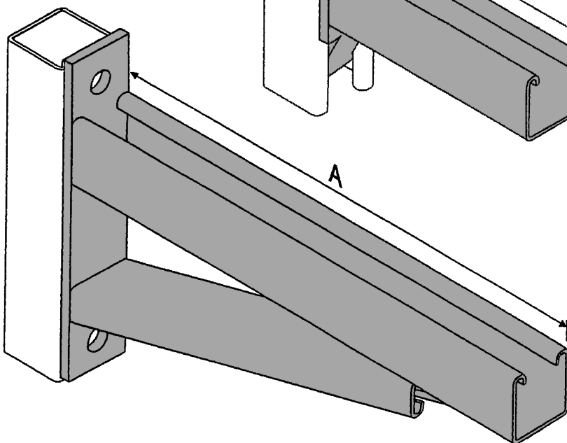
FM158 PIPE & CABLE CANTILEVER BRACKET PART NO. A FM158-150 150 FM158-300 300 FM158-450 450 FM158-600 600 FM158-780 780 FINISH: GALVANISED
