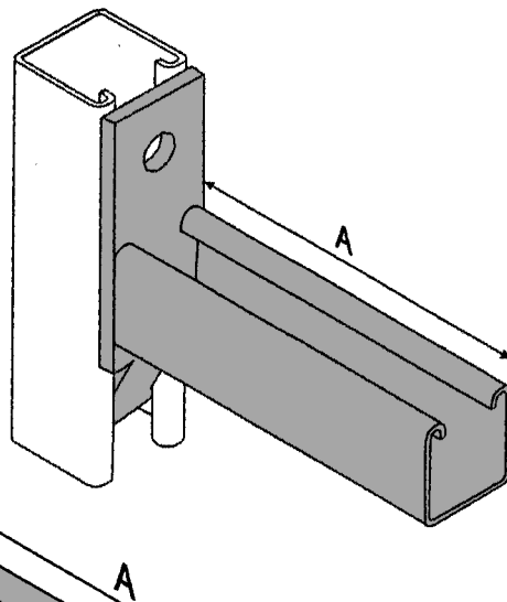
FM157 PIPE & CABLE CANTILEVER BRACKET PART NO. A FM157-150 150 FM157-300 300 FM157-450 450 FM157-600 600 FINISH: GALVANISED
